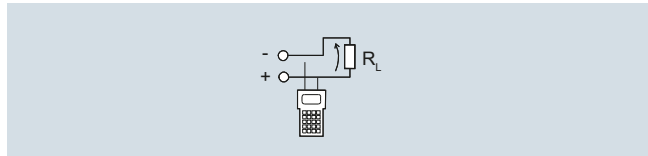
SITRANS I100 isolating power supply with HART, output configuration
