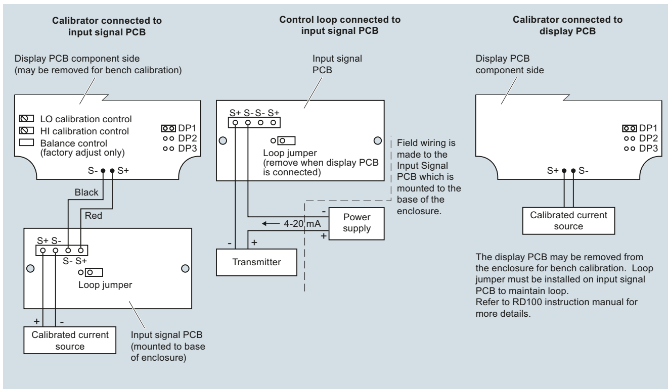
SITRANS RD100 connections
