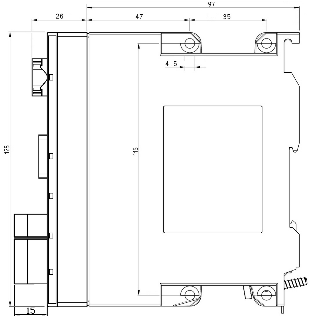
Figure 7-2 SCALANCE X101-1AUI side view
