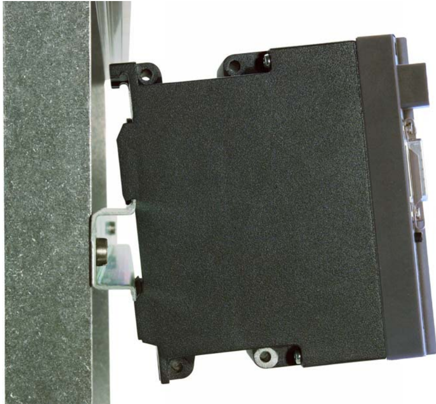
Figure 4-2 Removing from a DIN rail (35 mm)
