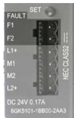
Figure 3-6 SCALANCE X101-1AUI signaling contact
