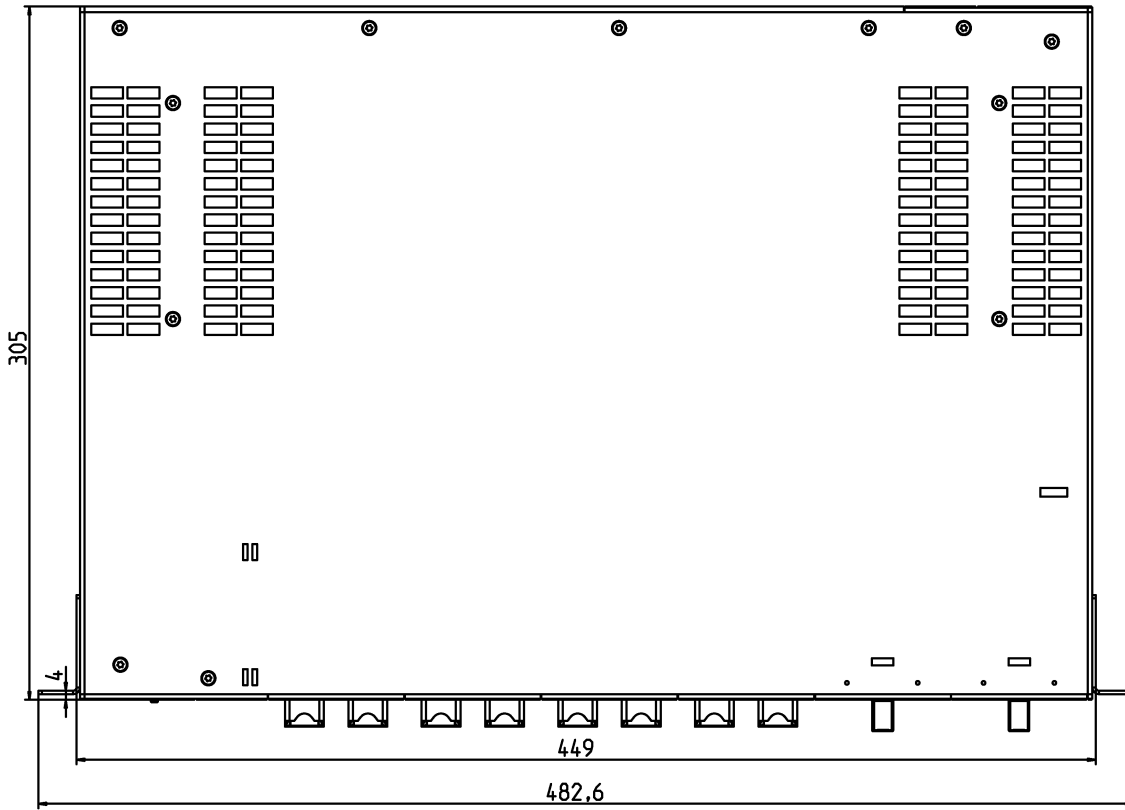
Image 7-4 XR324-4M PoE and XR324-4M PoE TS: From above
