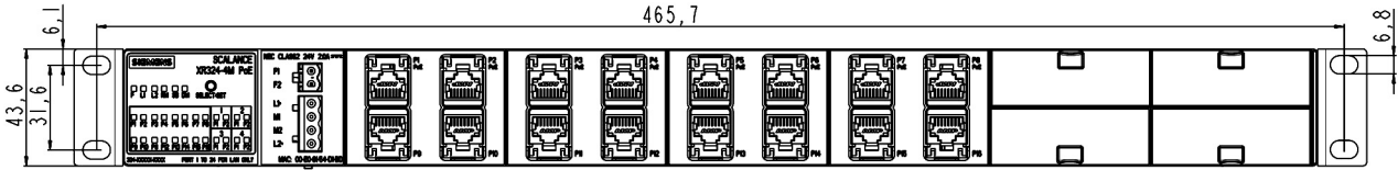
Image 7-1 XR324-4M PoE and XR324-4M PoE TS: Front view
