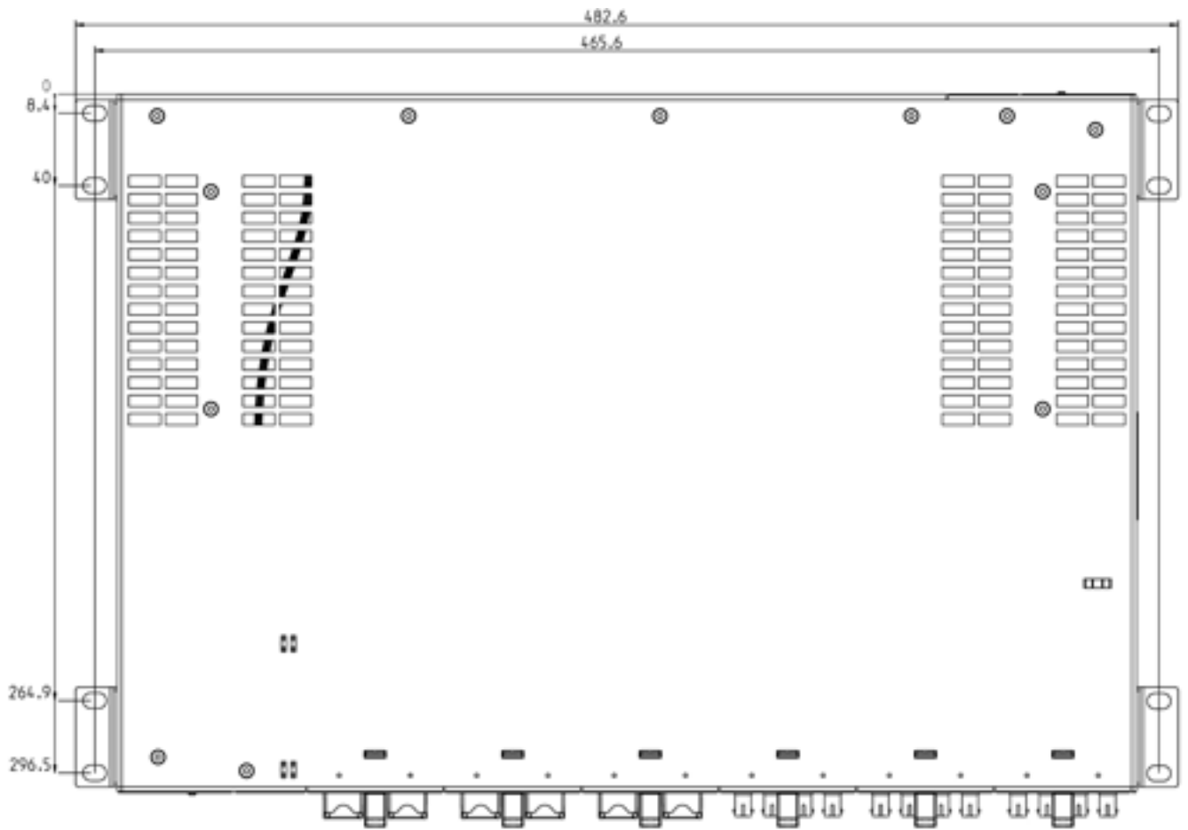
Image 7-3 XR324-12M from above
