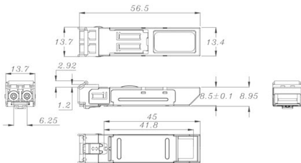
Image 11-29 SFP dimension drawing
