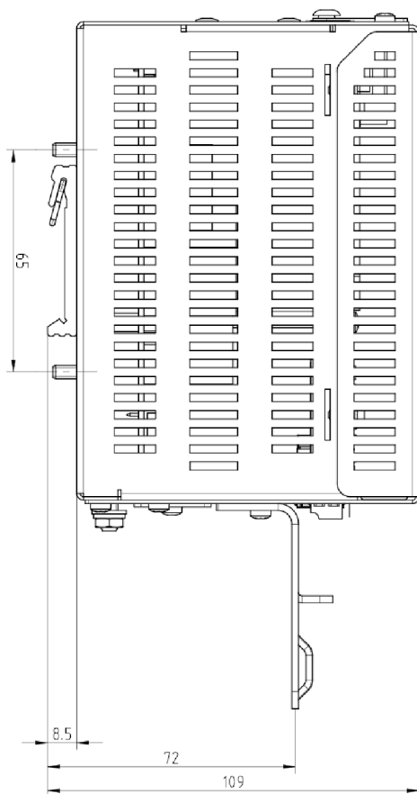
Image 11-14 Dimension drawing IE Switch X302-7EEC - side view
