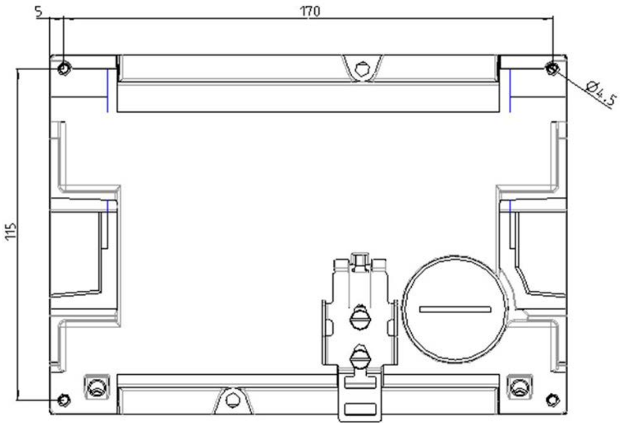
Image 11-7 Large design dimension drawing (IE Switch X-320)
