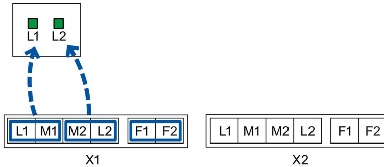
Image 6-2 Assignment of the LED display to the pins for redundant power supply with devices with two power supply units
