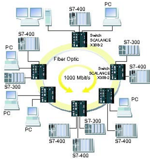
Image 3-4 Ring with FO cable and redundancy manager
