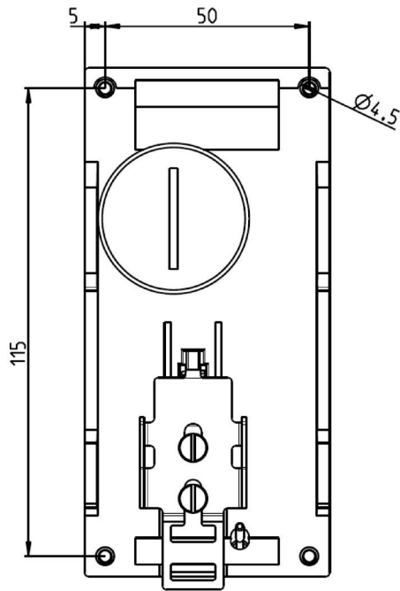
Image 11-2 Small design dimension drawing (IE Switch X-306)
