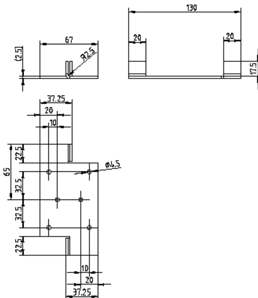
Image 11-21 Middle part of mounting support for X-300EEC (dimensions in mm)
