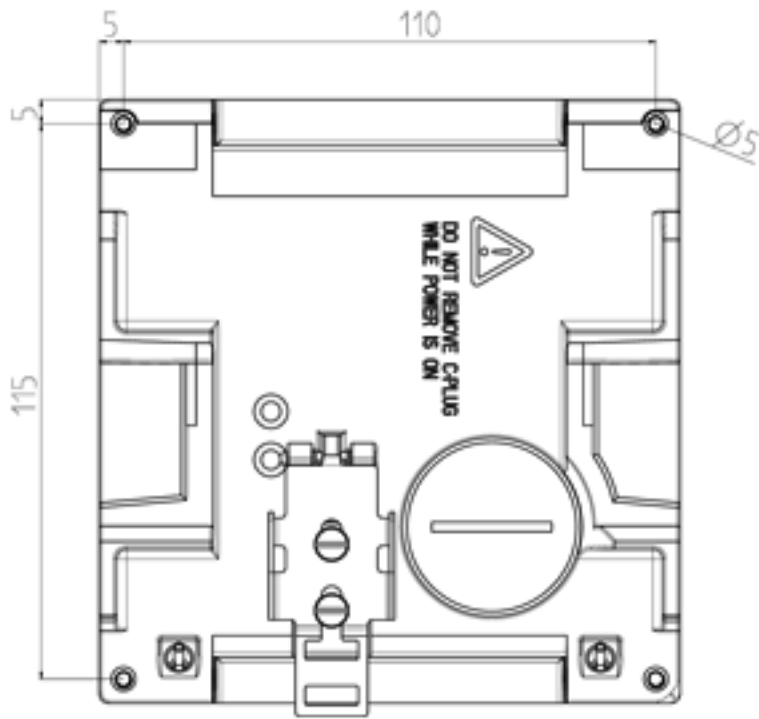
Image 11-9 X308-2M drilling template
