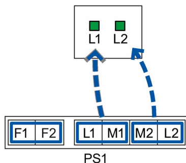
Image 6-4 Assignment of the LED display to the pins for redundant power supply with devices with one power supply unit
