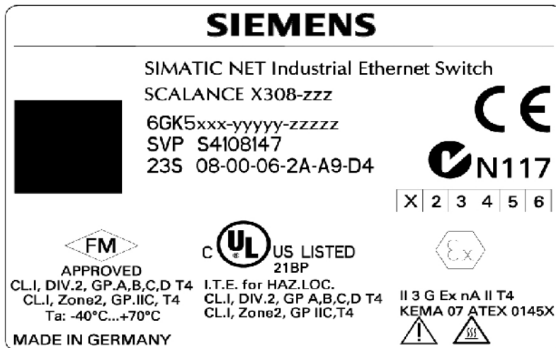
Image 9-3 Specimen X-300M type plate
