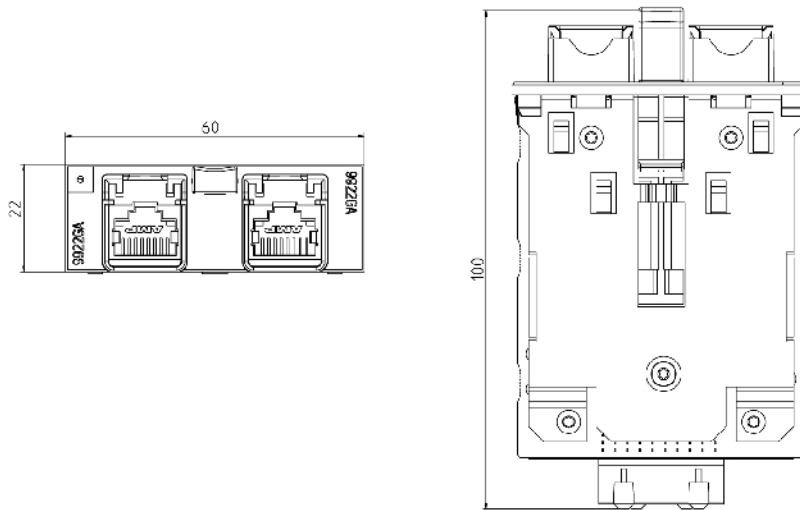
Image 11-22 MM900 dimension drawing 1: Electrical RJ-45 ports with securing collar
