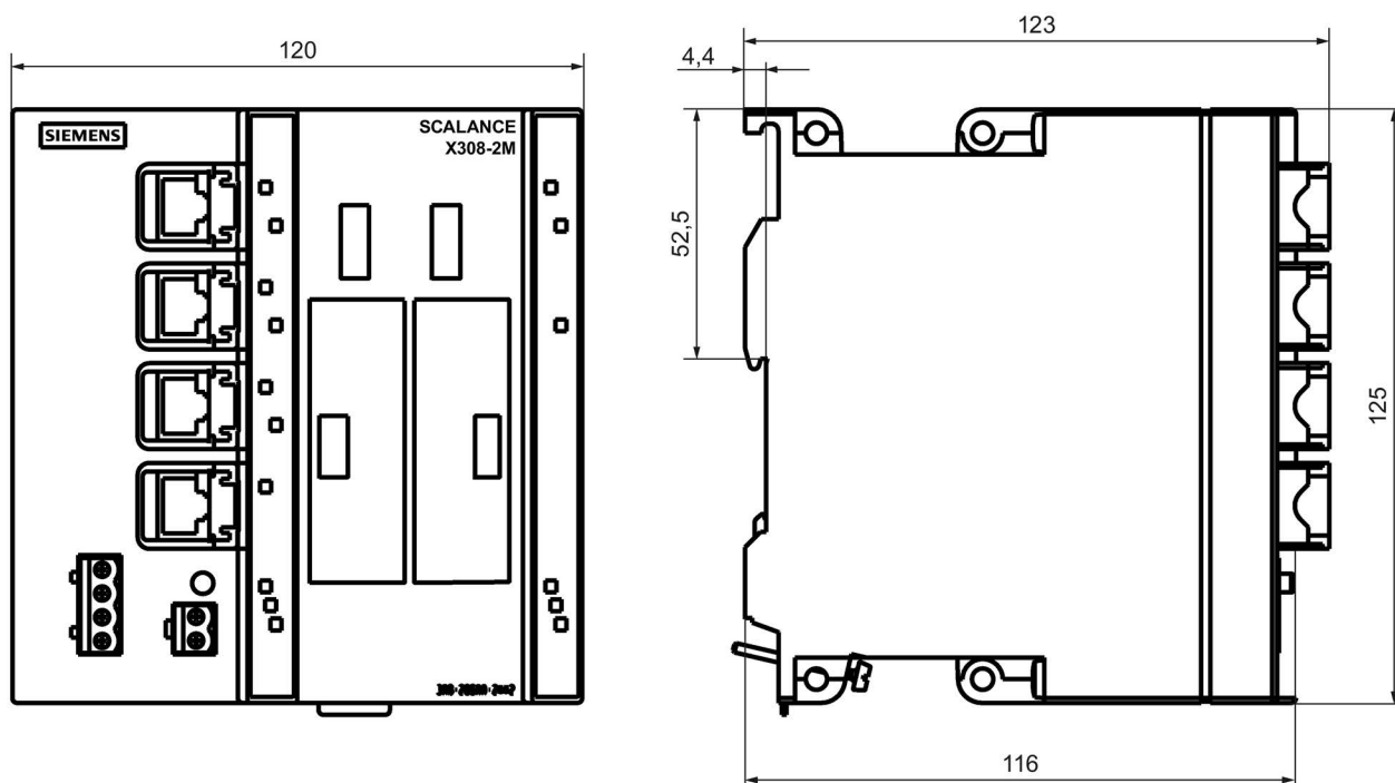
Image 11-8 X308-2M dimension drawing
