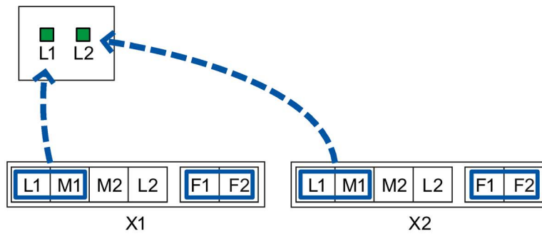
Image 6-3 Assignment of the LED display to the pins for redundant power supply with devices with two power supply units
