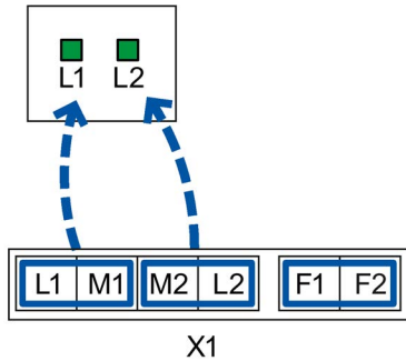
Image 6-1 Assignment of the LED display to the pins for redundant power supply with devices with one power supply unit
