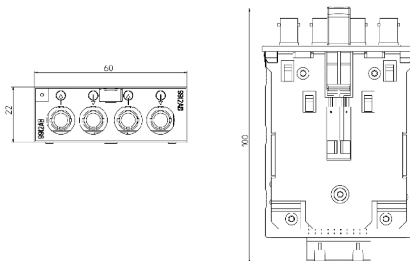
Image 11-24 MM900 dimension drawing 3: BFOC ports
