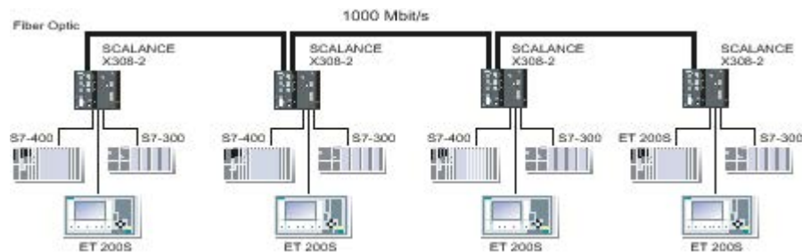
Image 3-1 Linear structure (optical)
