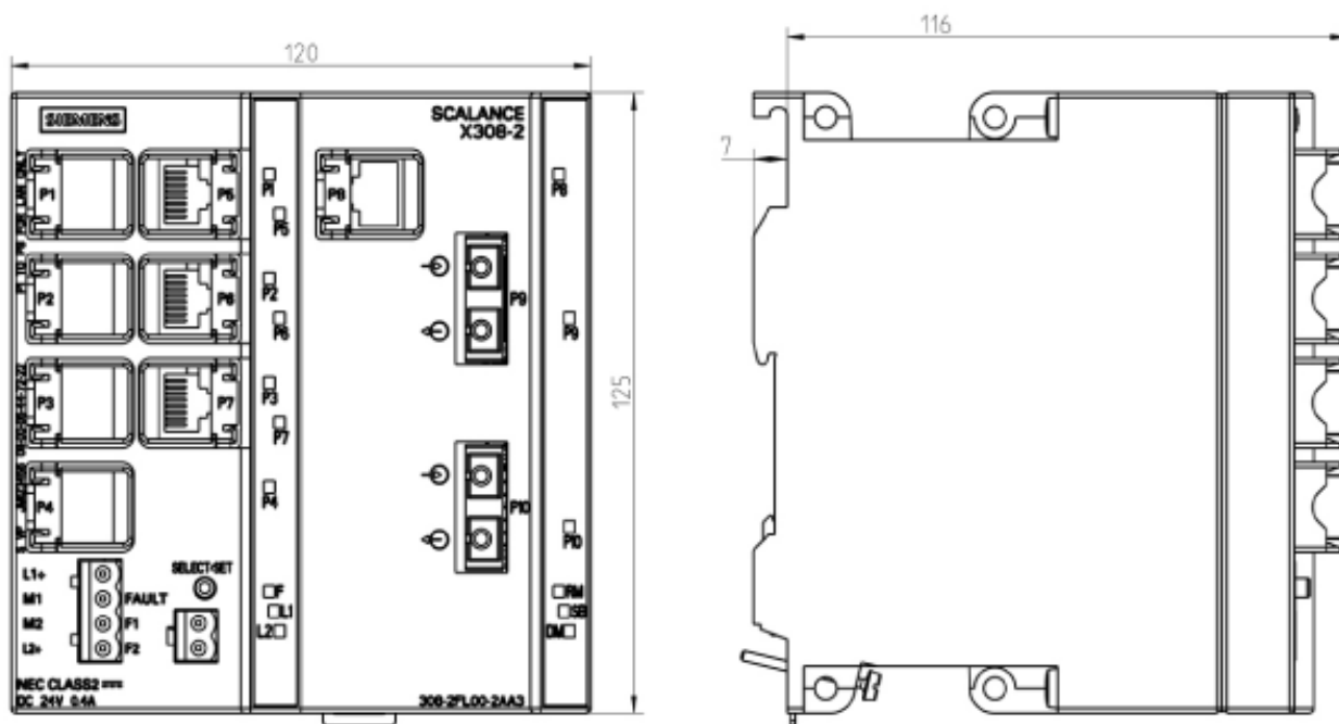
Image 11-3 Medium design dimension drawing (example used here SCALANCE X308-2)
