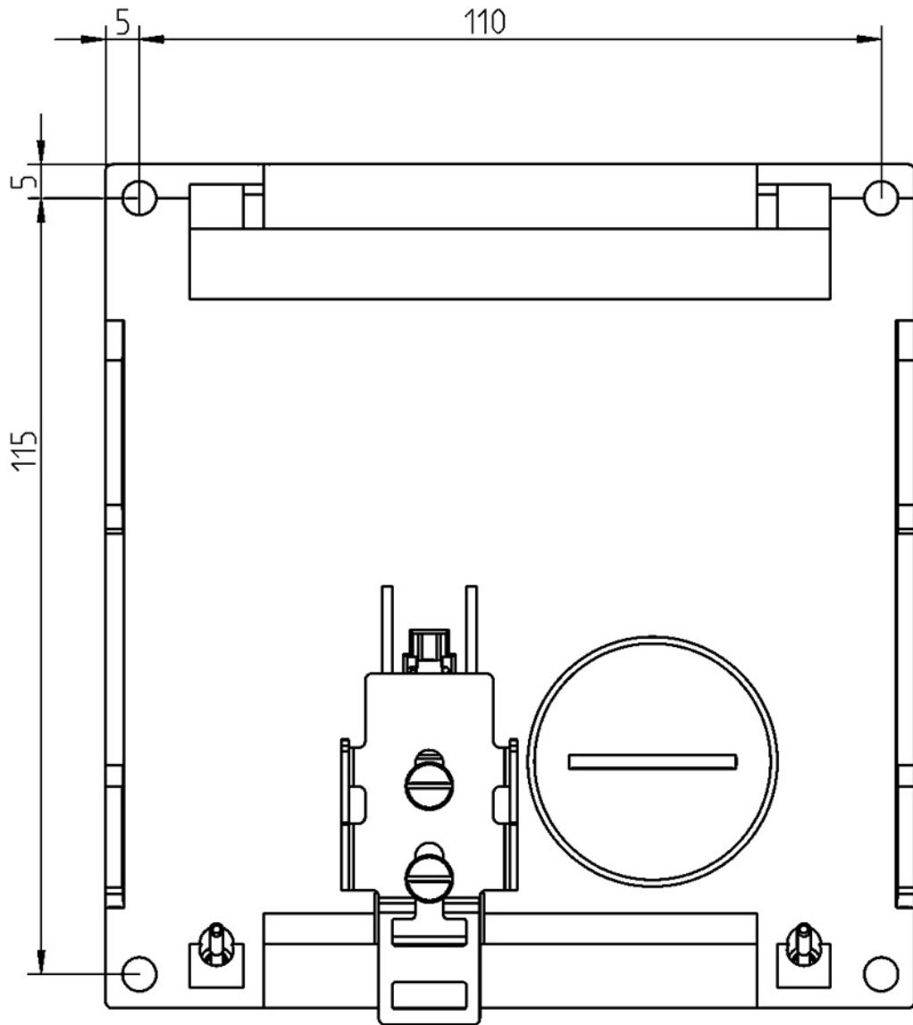
Image 11-32 X308-2M PoE: Drilling template
