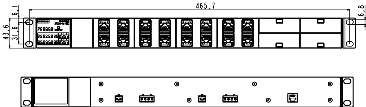
Image 11-16 Housing front and rear
