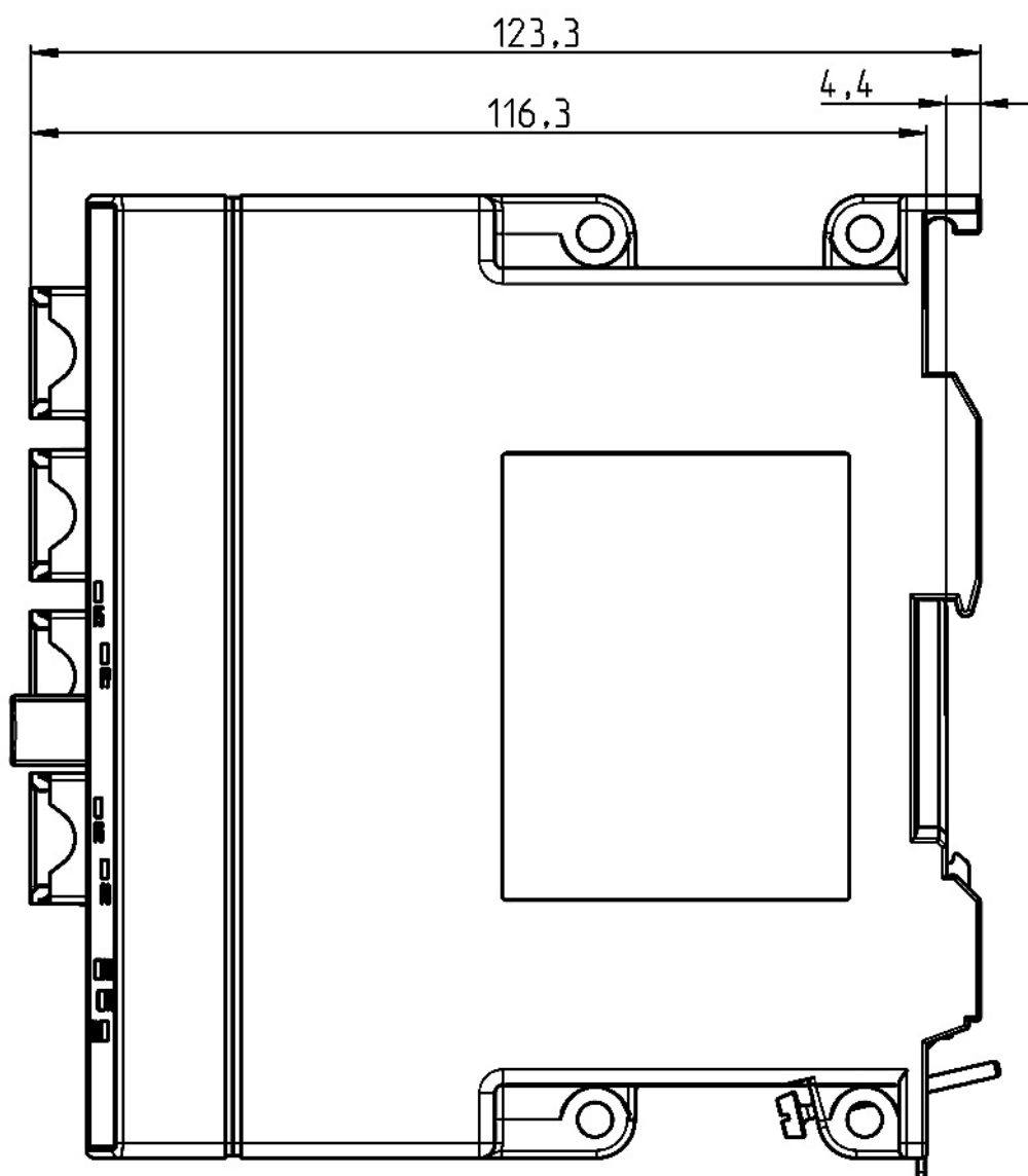
Image 11-31 X308-2M PoE: Side view
