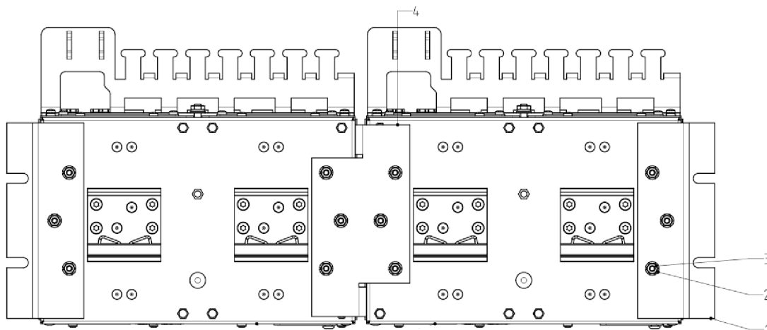
Image 11-19 Rack mounting of two X-300EECs fastened together (view from below)
