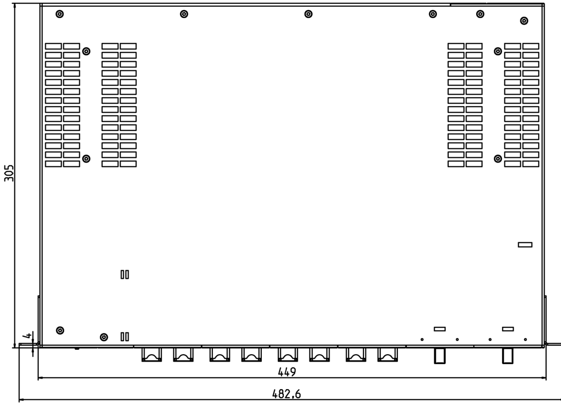
Image 11-36 XR324-4M PoE and XR324-4M PoE TS: From above
