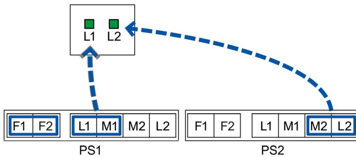
Image 6-6 Assignment of the LED display to the pins for redundant power supply with devices with two power supply units.
