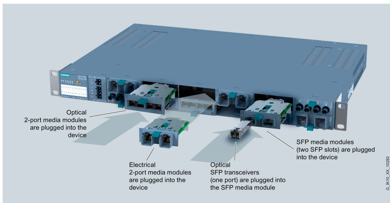
Image 2-1 Designs of the X-300 IE switches, example of plugging media modules into the media module slots of the XR324-12M
