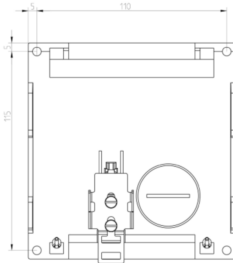
Image 11-4 Medium design dimension drawing (IE Switch X-300)
