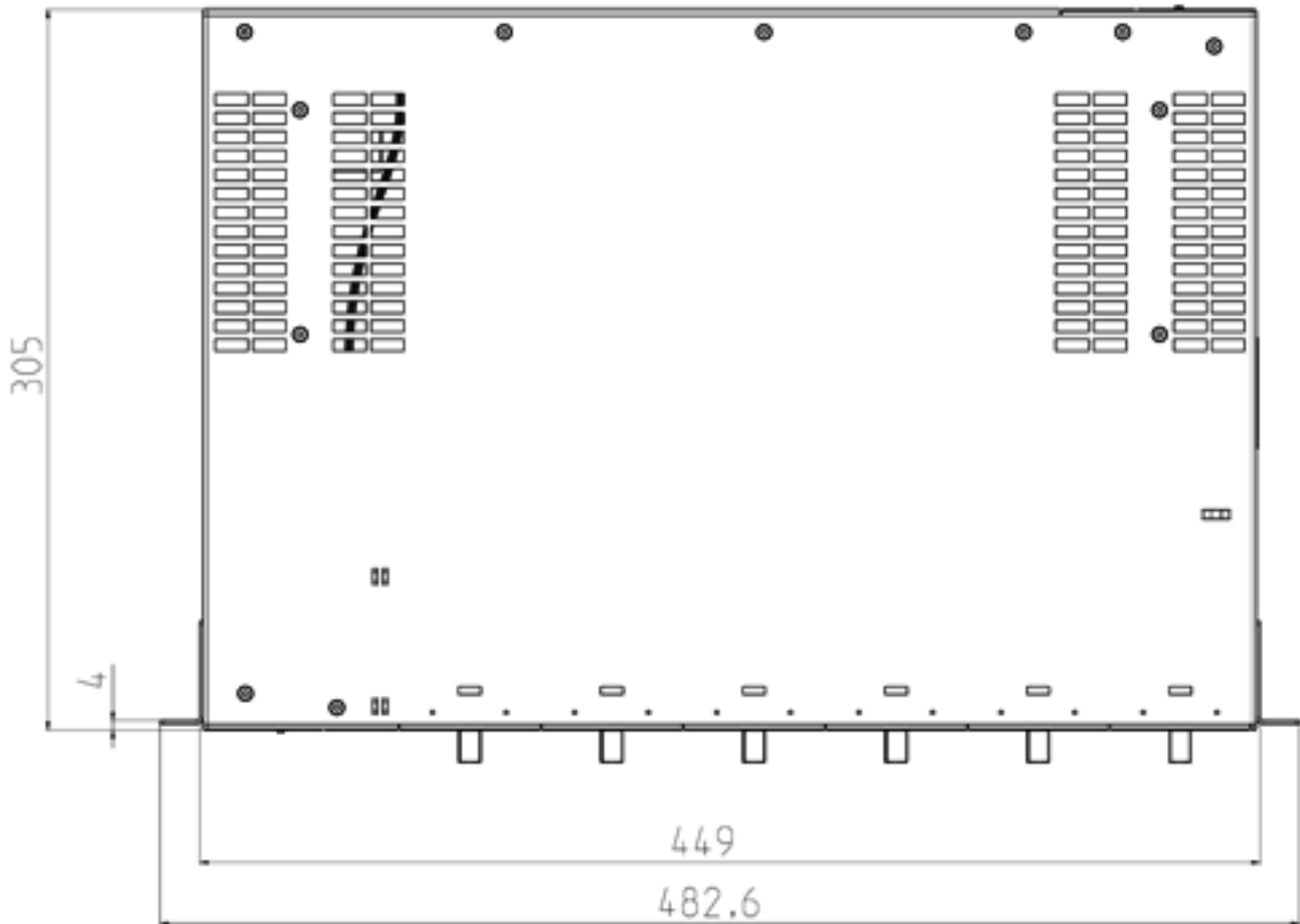
Image 11-11 XR324-12M from above
