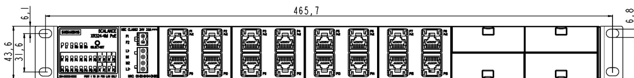
Image 11-33 XR324-4M PoE and XR324-4M PoE TS: Front view
