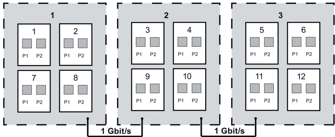
Image 8-3 Block architecture of the XR324-12M
