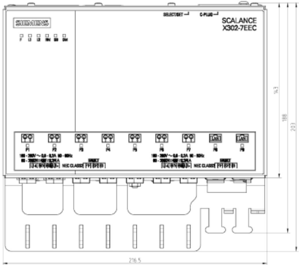
Image 11-13 Dimension drawing IE Switch X302-7EEC - view
