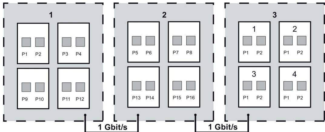
Image 8-2 Block architecture of the XR324-4M
