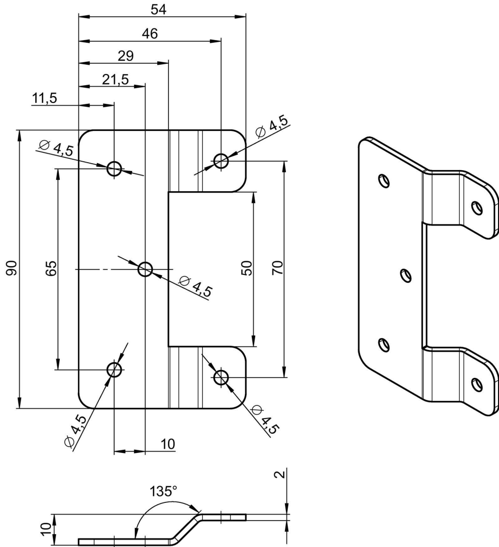
Image 11-18 X-300EEC wall mounting (dimensions in mm)
