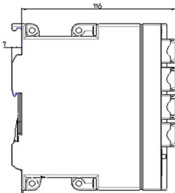
Image 11-6 Large design dimension drawing Part 2 (example used here SCALANCE X320-3LD FE)
