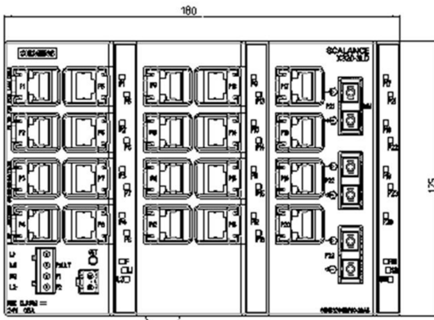
Image 11-5 Large design dimension drawing Part 1 (example used here SCALANCE X320-3LD FE)
