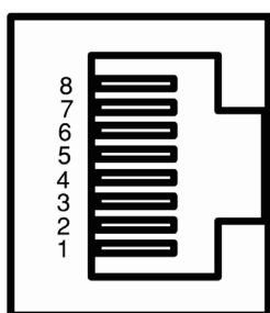
Image A-1 RJ-45 jack
