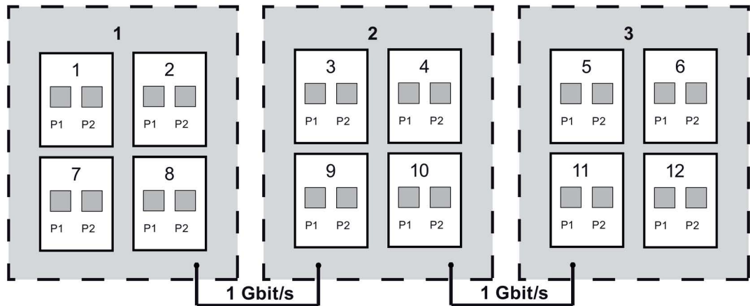
Image 8-1 Block architecture of the XR324-12M
