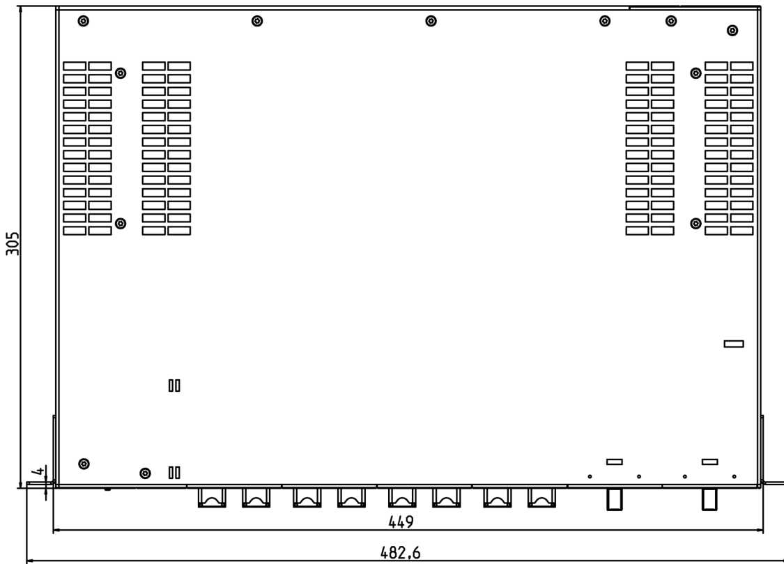
Image 11-17 Top of the housing
