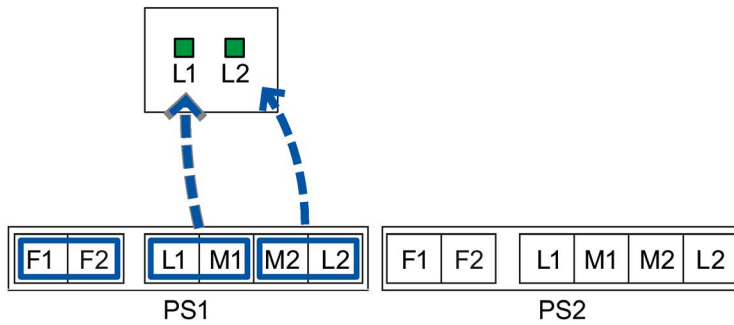
Image 6-5 Assignment of the LED display to the pins for redundant power supply with devices with two power supply units
