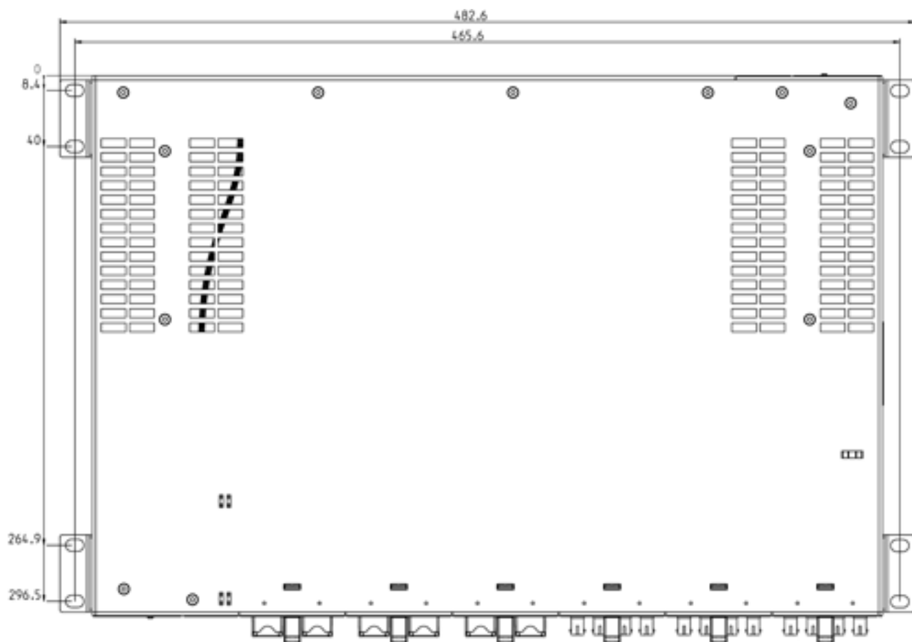
Image 11-12 XR324-12M from above
