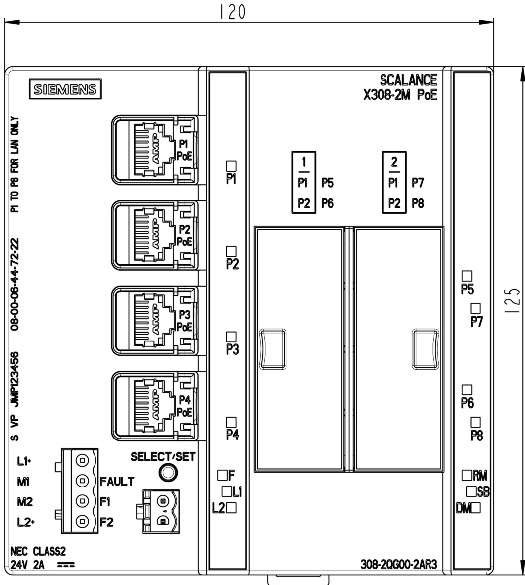
Image 11-30 X308-2M PoE: Front view
