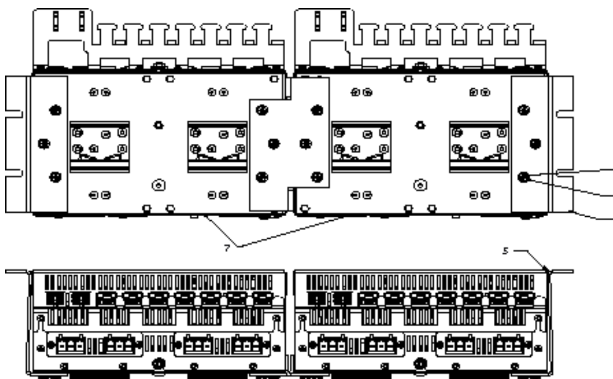
Image 5-4 Rack mounting of two IE-Switches X-300EEC fastened together Figure at top: Rear of the switches Figure at bottom: View from below
