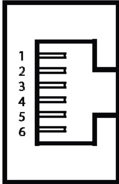
Image 7-2 RJ-11 jack (schematic)
