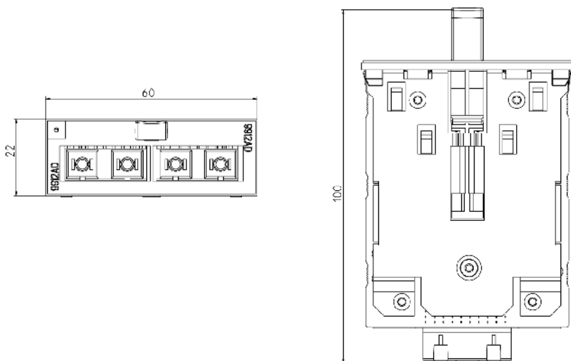
Image 11-25 MM900 dimension drawing 4: Optical SC ports
