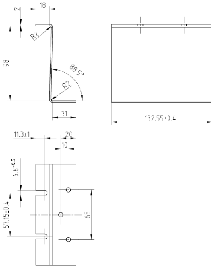
Image 11-20 Side part of mounting support for X-300EEC (dimensions in mm)
