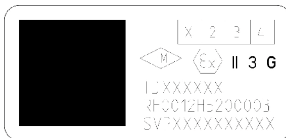
Image 9-9 SFP specimen type plate bottom
