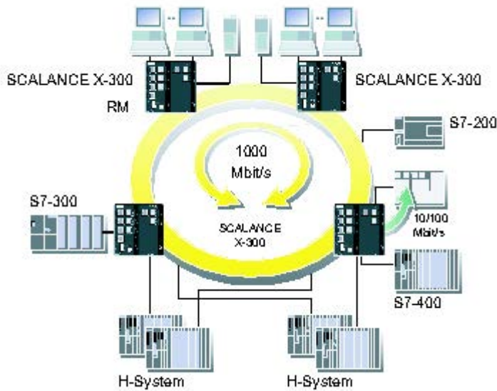
Image 3-3 Gigabit ring with redundancy manager (RM)
