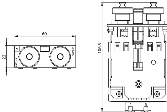
Image 11-27 MM900 dimension drawing 6: M12 ports electrical
