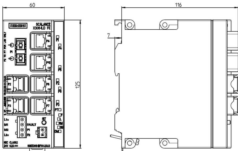
Image 11-1 Small design dimension drawing (example used here SCALANCE X306-1LD FE)
