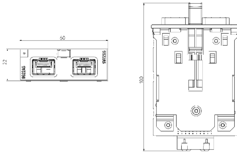
Image 11-26 MM900 dimension drawing 5: SFP media module
