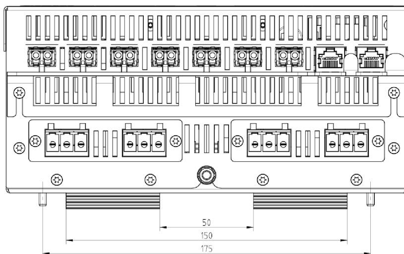
Image 11-15 Dimension drawing IE Switch X302-7EEC - from above
