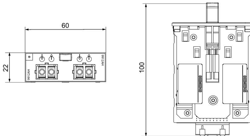
Image 11-28 MM900 dimension drawing 7: SC RJ ports optical
