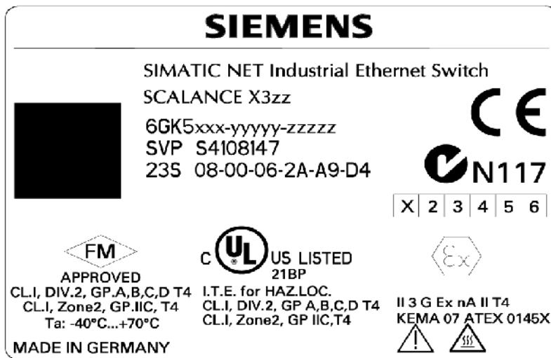
Image 9-1 X-300 specimen type plate
