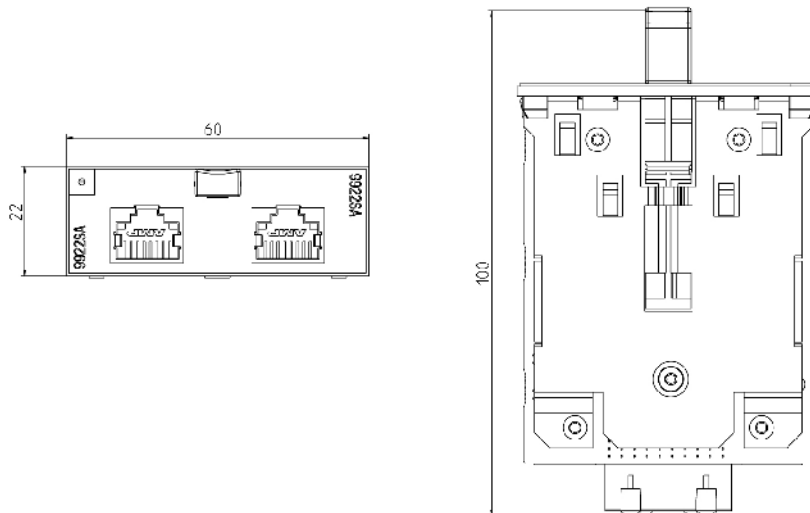
Image 11-23 MM900 dimension drawing 2: Electrical RJ-45 ports without securing collar
