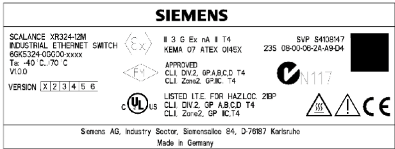
Image 9-5 Specimen XR-300M type plate
