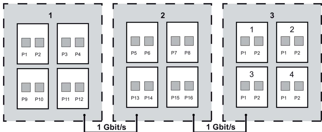
Image 8-5 Block architecture of the XR324-4M
