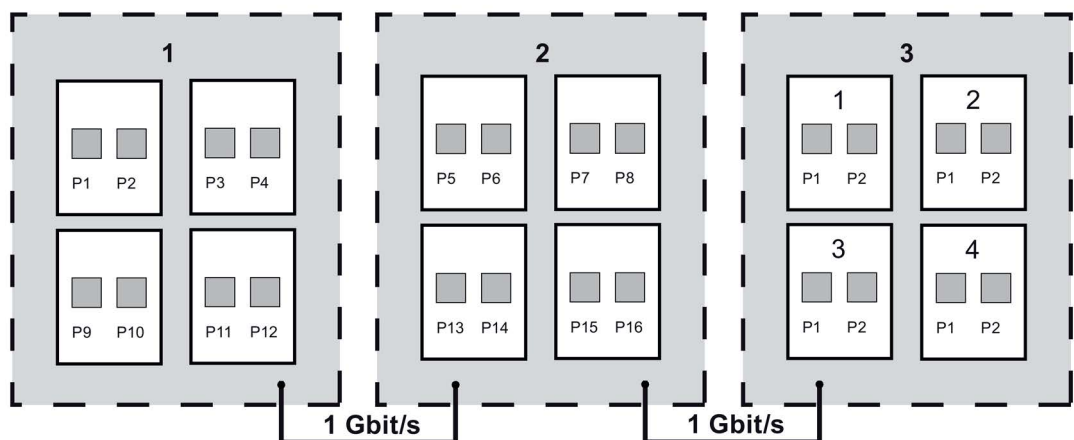
Image 8-4 Block architecture of the XR324-4M
