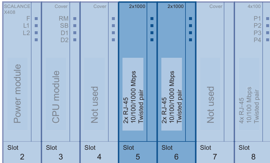
Figure 3-2 Slots of the media modules
