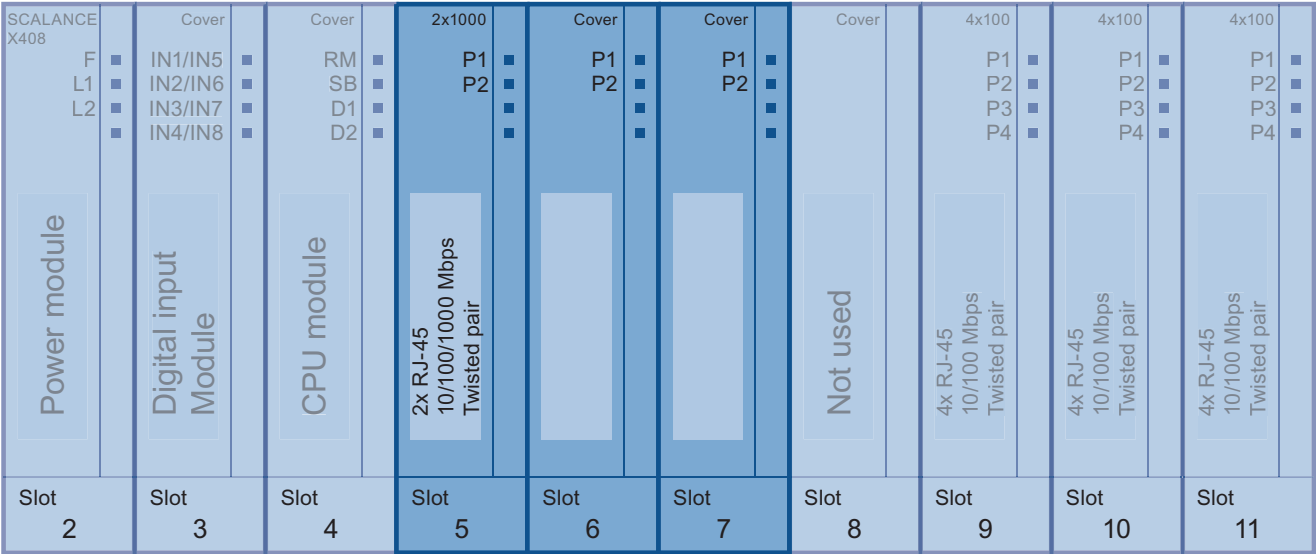
Figure 3-1 Slots of the media modules
