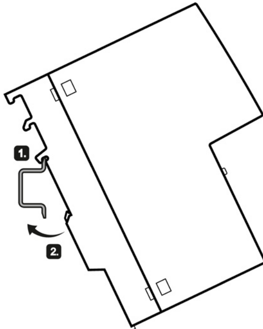
Figure 4-1 DIN rail mounting
