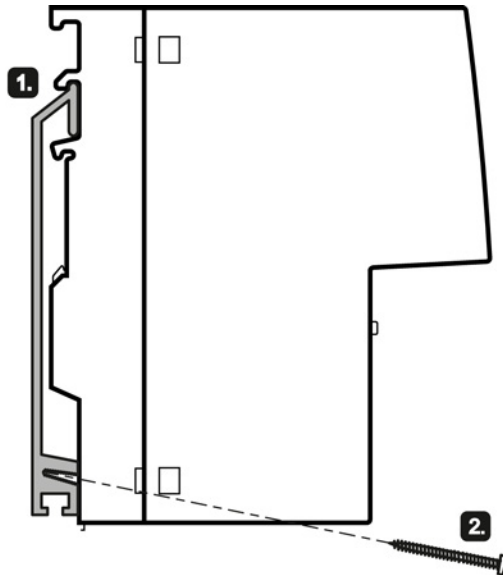
Figure 4-2 S7-300 standard rail mounting
