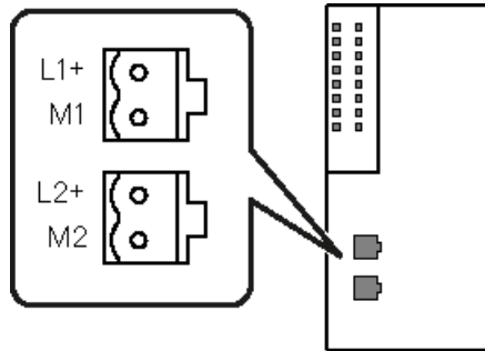
Figure 5-1 Position of the PoE power supply on the PE408PoE and the assignment of the terminal blocks
