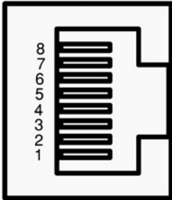
Figure 3-1 RJ-45 jack
