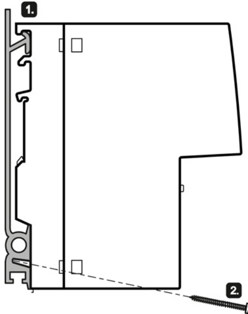
Figure 4-3 S7-1500 standard rail mounting
