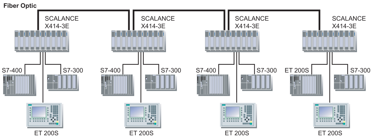
Figure 3-1 Linear structure (optical)
