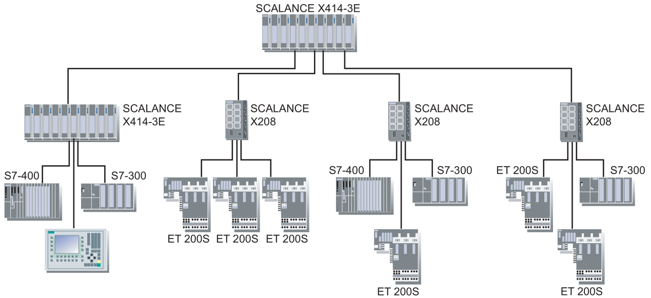
Figure 3-2 Star structure (electrical)
