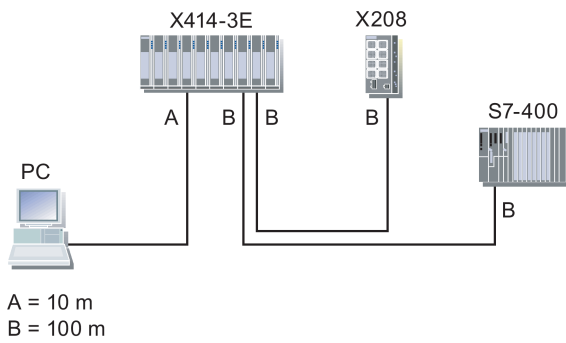
Figure 5-5 FastConnect cabling A TP cord (1 Gbps) B IE FC standard cable 2x2 (100 Mbps)
