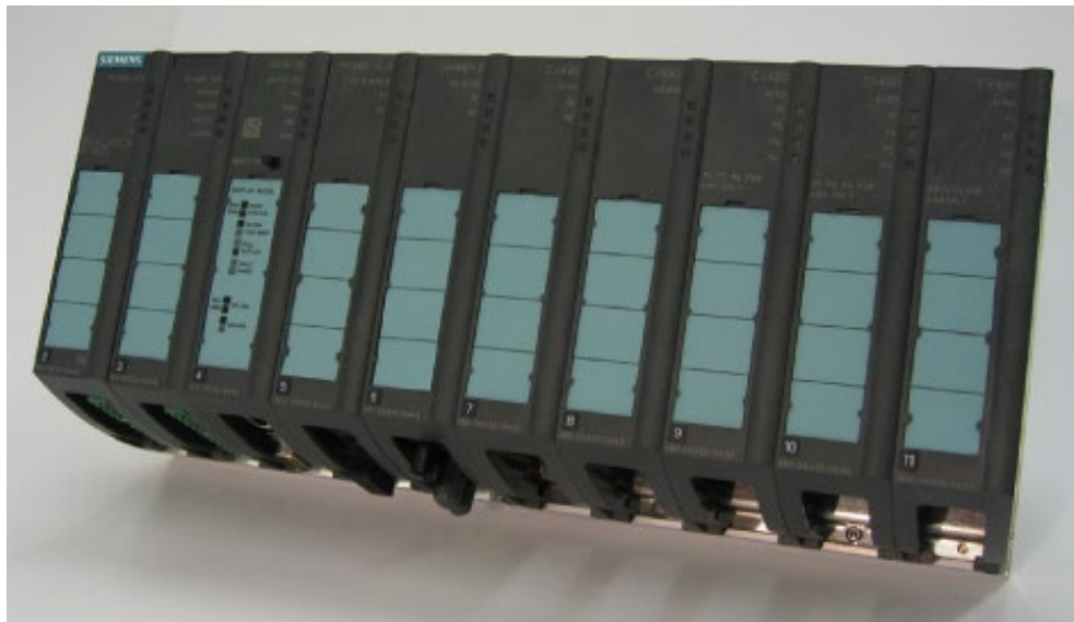
Figure 3-9 Basic device with media modules and covers
