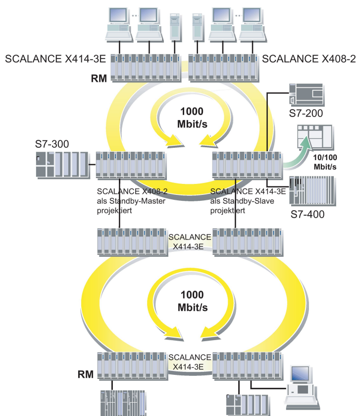
Figure 3-7 Redundant coupling of two subnets in mixed operation with SCALANCE X414-3E and SCALANCE X408-2
