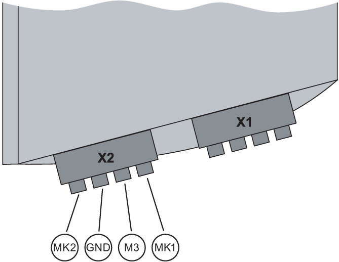
Figure 5-2 Pins of connector X2
