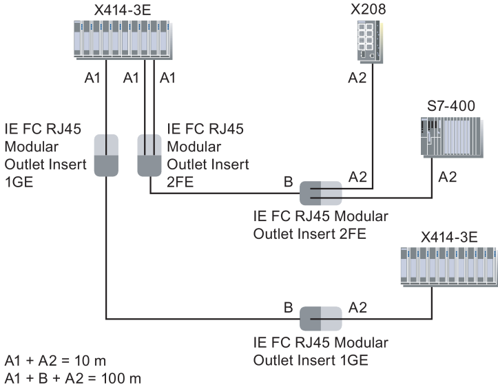
Figure 5-8 FastConnect cabling A1 TP cord 4x2 A2 TP cord 4x2 B IE FC standard cable 4x2
