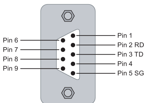
Figure 3-22 Pin assignment of the serial interface
