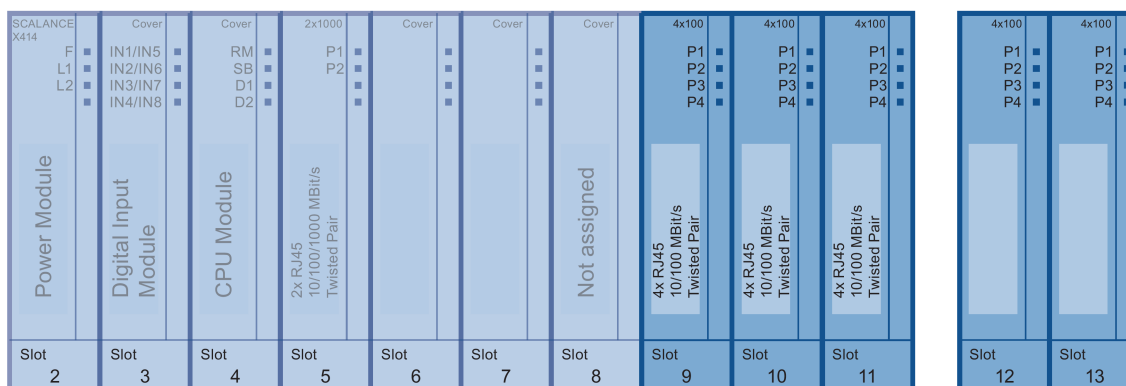
Figure 3-38 Slots 12 and 13 for the CV490 4x100 cover on the twisted pair extender module EM495-8
