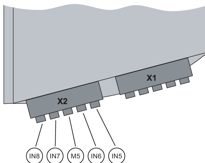
Figure 5-4 Pins of connector X2 (inputs 5-8)
