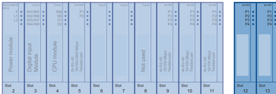
Figure 3-27 Basic device with twisted pair extender module
