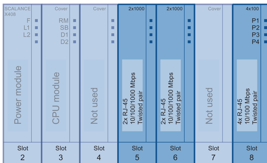
Figure 3-40 Possible slots of the covers
