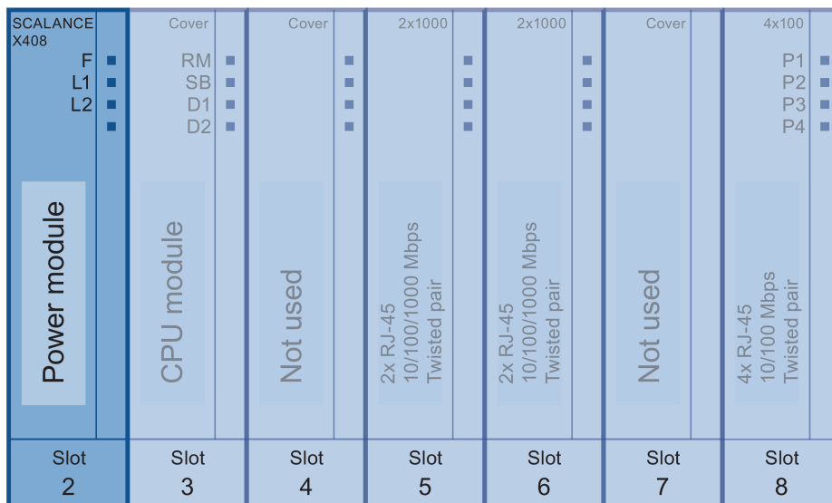
Figure 3-20 Slot of the power module
