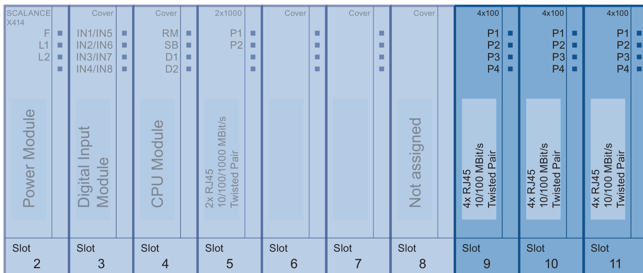
Figure 3-37 Slots 9 to 11 for CV490 4x100 cover
