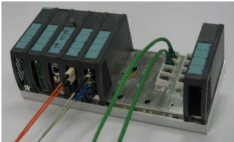
Figure 3-16 Basic device with gigabit fiber-optic cable and Fast Ethernet twisted-pair cable
