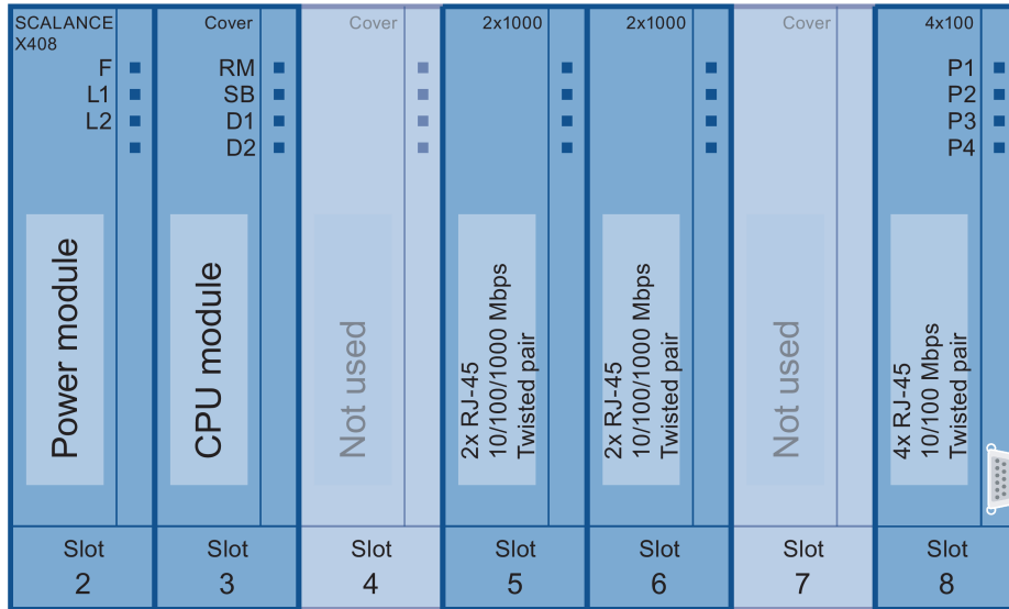
Figure 3-19 Basic device X408-2 without media modules with existing ports
