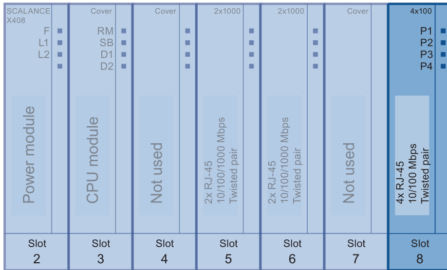
Figure 3-42 Slot 8 for the CV 490 4x100 cover
