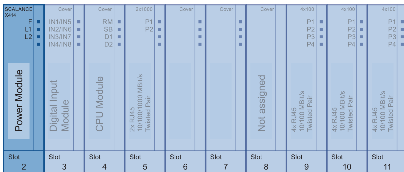
Figure 3-11 Slot of the power module
