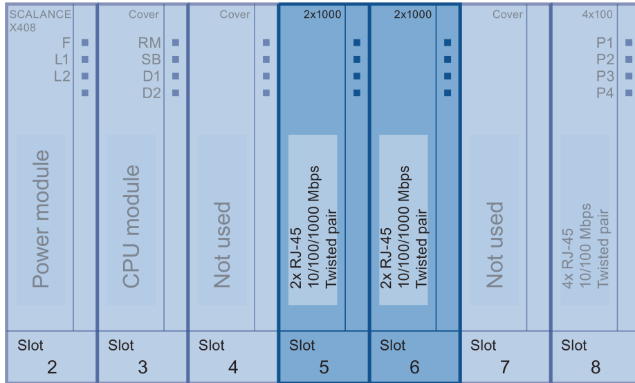
Figure 3-41 Slots 5 and 6 for cover CV490 2x1000
