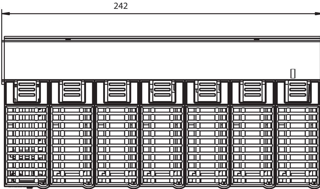
Figure 9-5 SCALANCE X408 top
