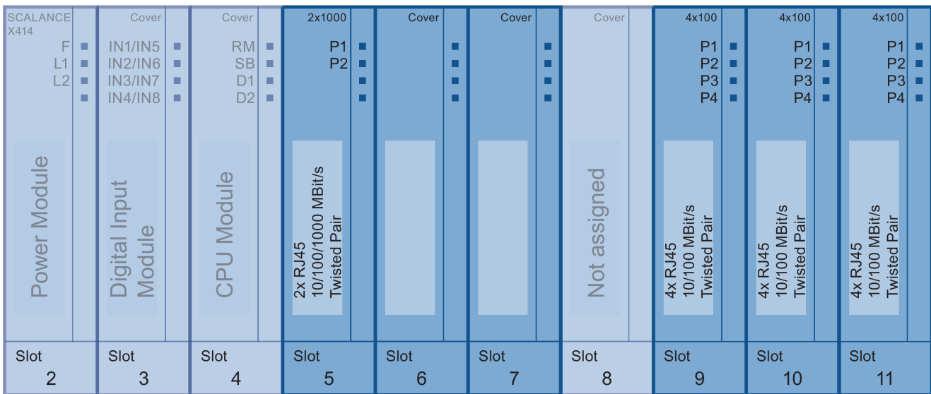
Figure 3-33 Possible slots of the covers
