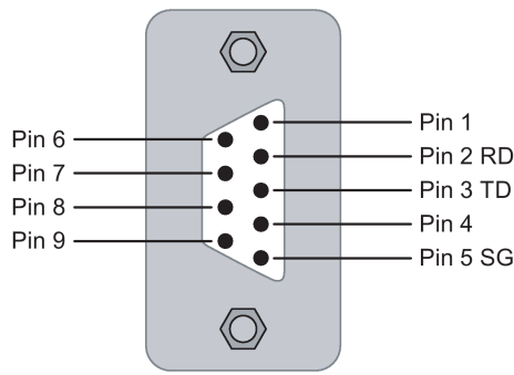
Figure 3-14 Pin assignment
