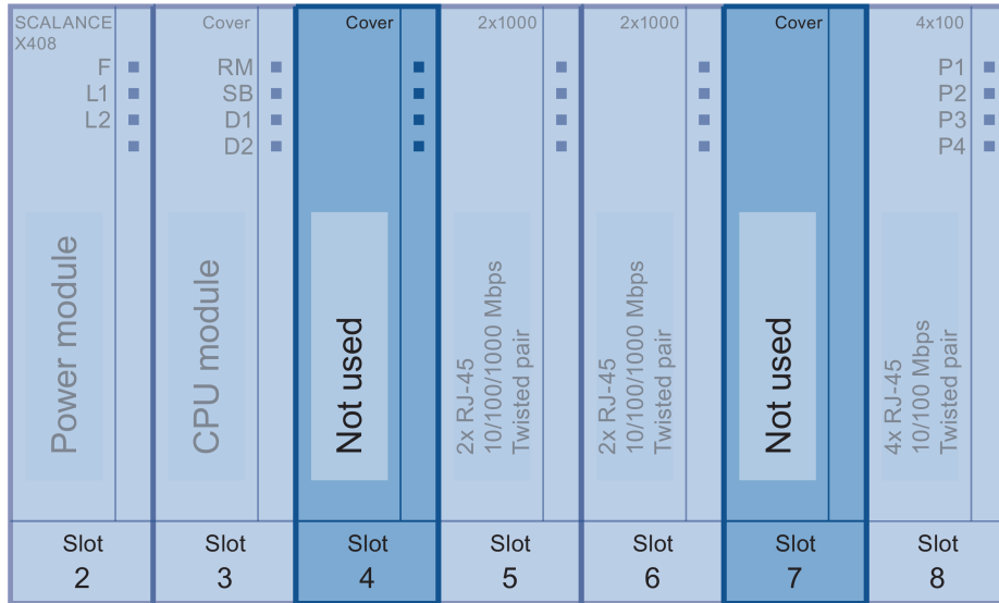
Figure 3-43 Slot 4 and 7 of the dummy cover SCALANCE X408-2
