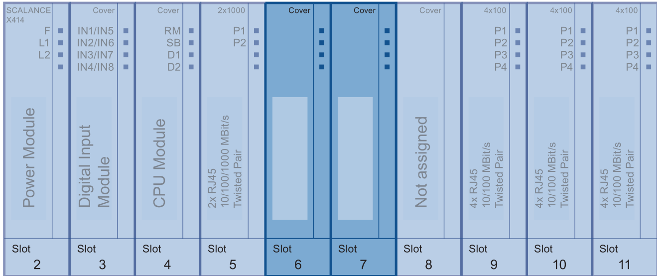
Figure 3-35 Slots 6 and 7 for the CV490 2x100 cover
