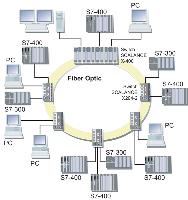
Figure 3-5 Optical ring with redundancy manager
