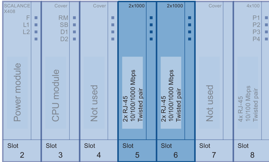
Figure 3-26 Slots of the media modules
