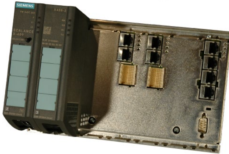
Figure 3-17 SCALANCE X408-2 basic device without media modules, protective caps and covers
