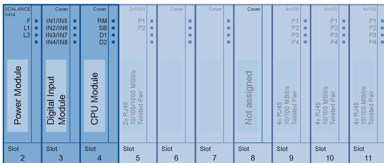
Figure 3-10 Basic device X414-3E without media modules with existing ports
