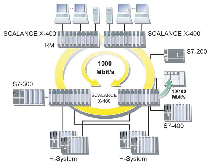
Figure 3-4 Gigabit ring with redundancy manager (RM)
