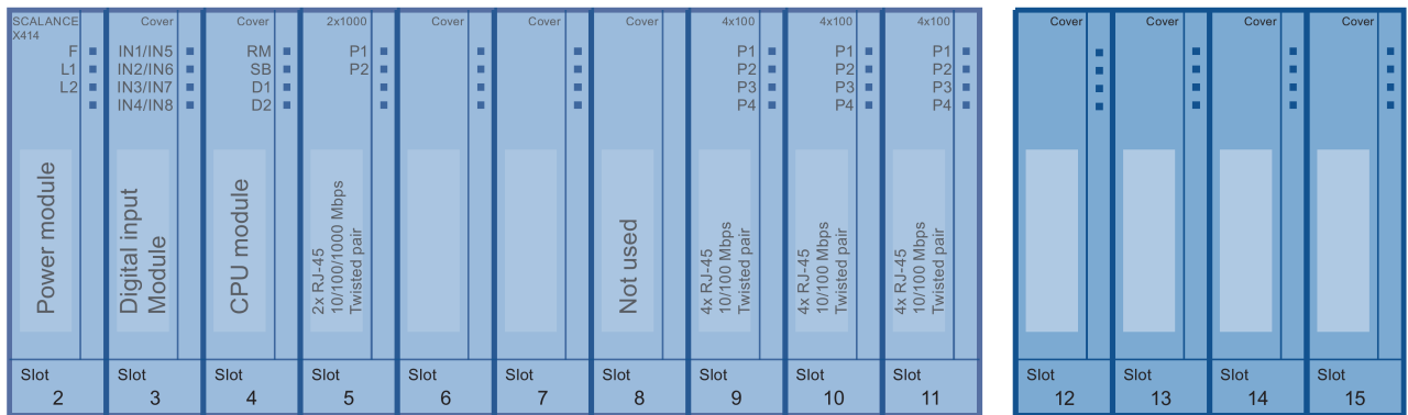
Figure 3-36 Slots 12 through 15 for CV490 2x100 cover on media module extender EM496-4
