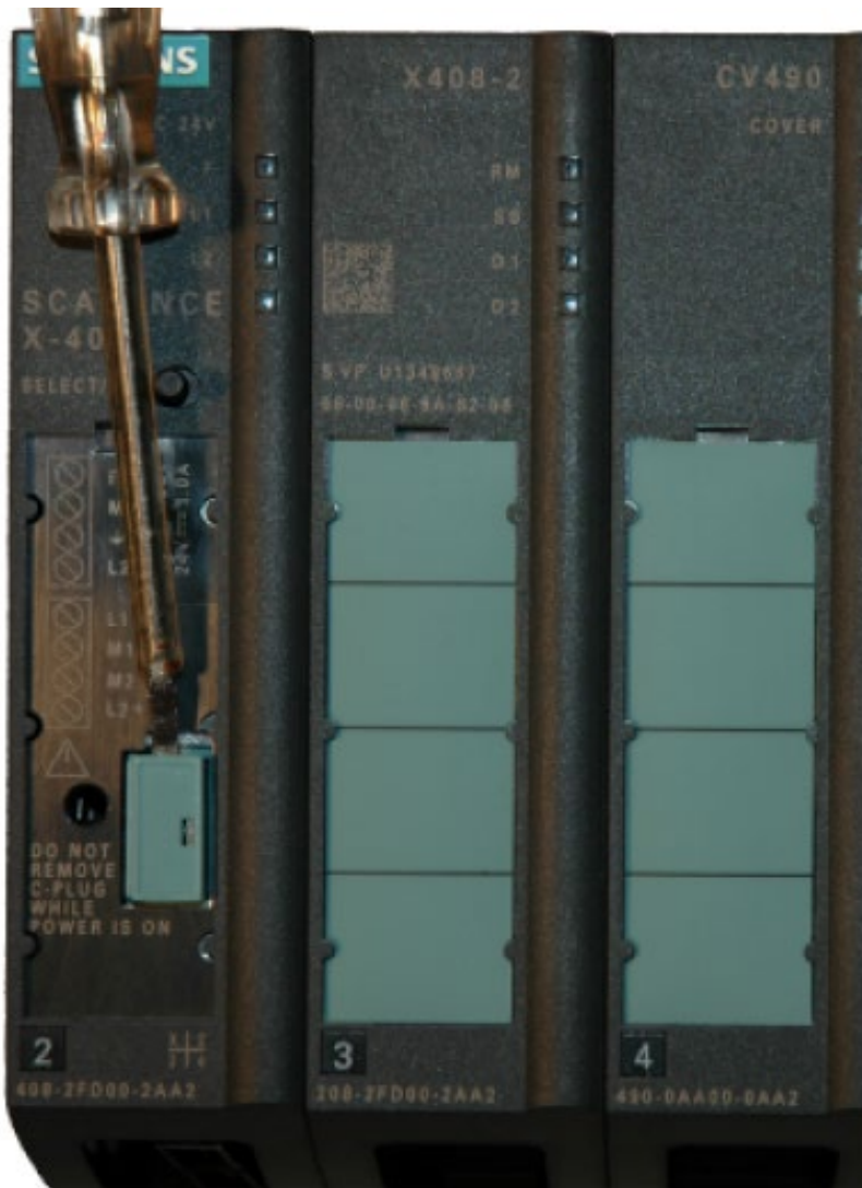
Figure 6-14 Removing the C-PLUG from the SCALANCE X408-2
