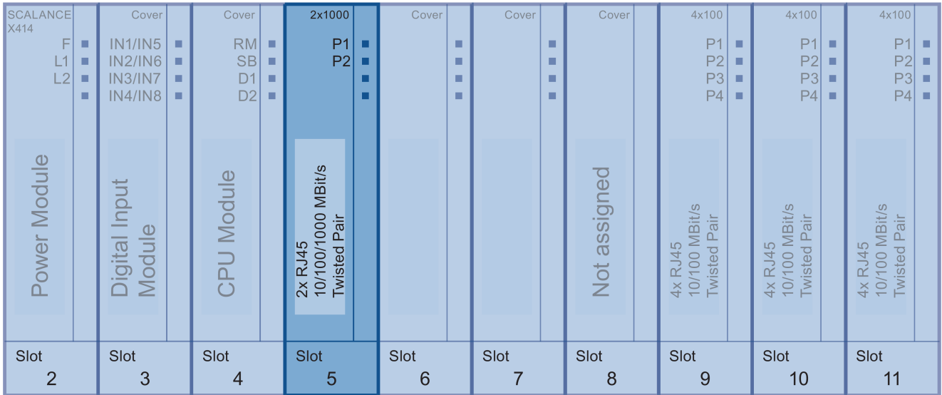
Figure 3-34 Slot 5 for the CV490 2x1000 cover
